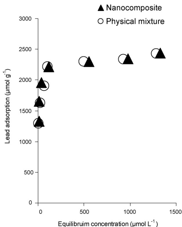
Fig. 6. Pb adsorption isotherms of nanocomposite sample and LTA-goethite mixture. 50 mg of sample was mixed with 30 mL of 0–5 mM \text{Pb}(\text{NO}_3)_2 , and shaken at 20 \pm 1^\circ\text{C} for 24 h. pH was maintained at 5.00 \pm 0.02 throughout the experiment.
