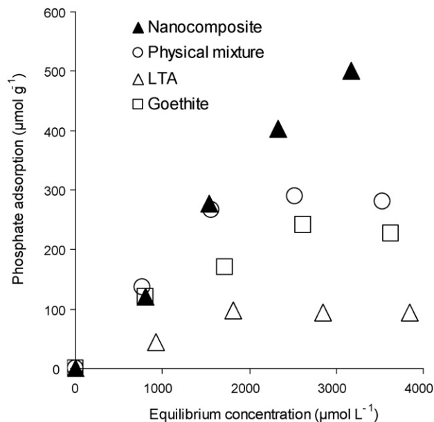
Fig. 7. Phosphate adsorption isotherms of nanocomposite sample, LTA-goethite mixture, synthetic LTA, and synthetic goethite. 50 mg of sample was mixed with 30 mL of 0–4 mM \text{NaH}_2\text{PO}_4 , and shaken at 20 \pm 1^\circ\text{C} for 24 h.
